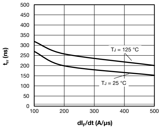
Fig. 14 - Typical D1 to D2 Antiparallel Diode Reverse Recovery Time vs. di_F/dt
